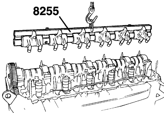
Fig. 5: Removing the rocker arm shaft assembly
