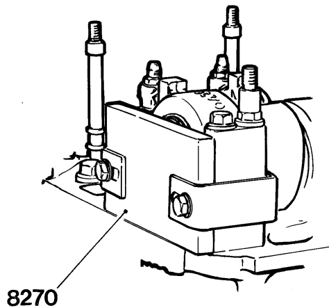
Fig. 7: Tool 9998270 installed
