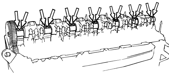
Fig. 13: Tightening rocker arm shaft and camshaft together
