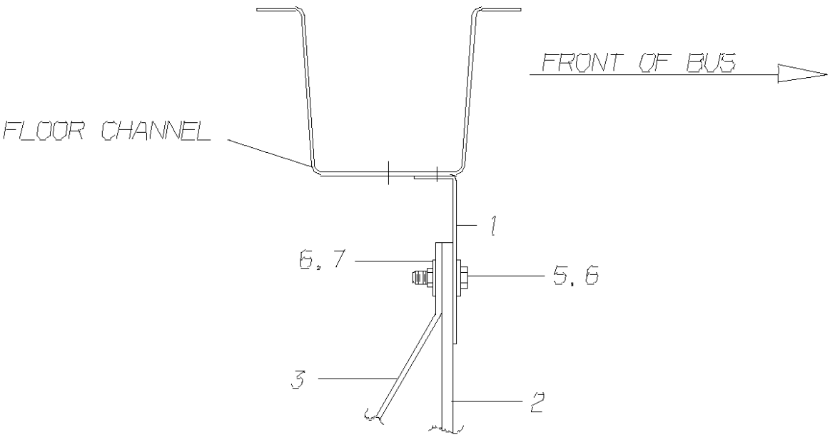
ALL A1/B1/B2VC EXCEPT FORD B2VC
