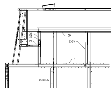
DETAIL F TUBE ASSY, SUPPORT, TRANSITION, MOUNTING LOCATION DETAIL
