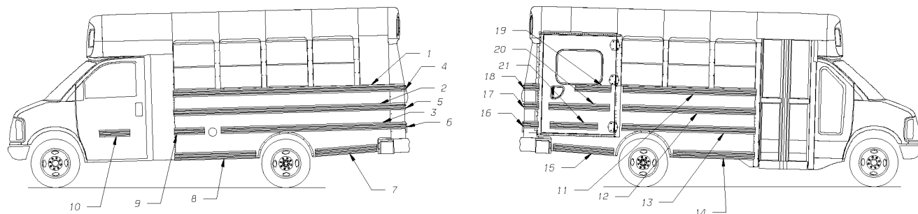
AFFD/GM 1502 BODY WITH LIFT
