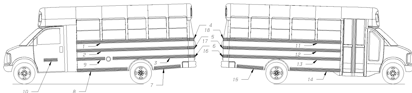
AFGM 1611 BODY WITHOUT LIFT
