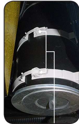
A3FE Air Filter mounting clamps
