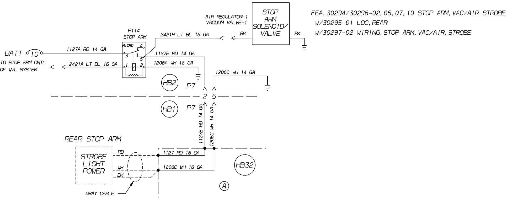
Stop Arm, Vac/Air, Strobe, Feature 30297-02, 0027671 A
