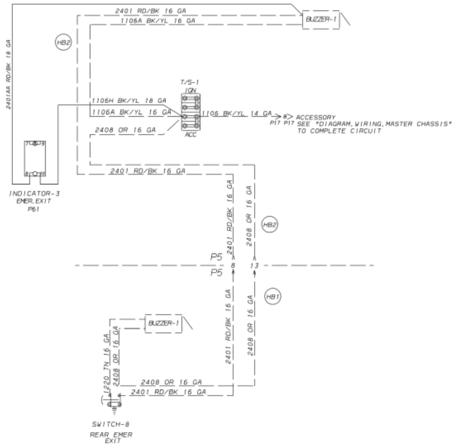
EMERGENCY EXIT PILOT LIGHT 0028508
