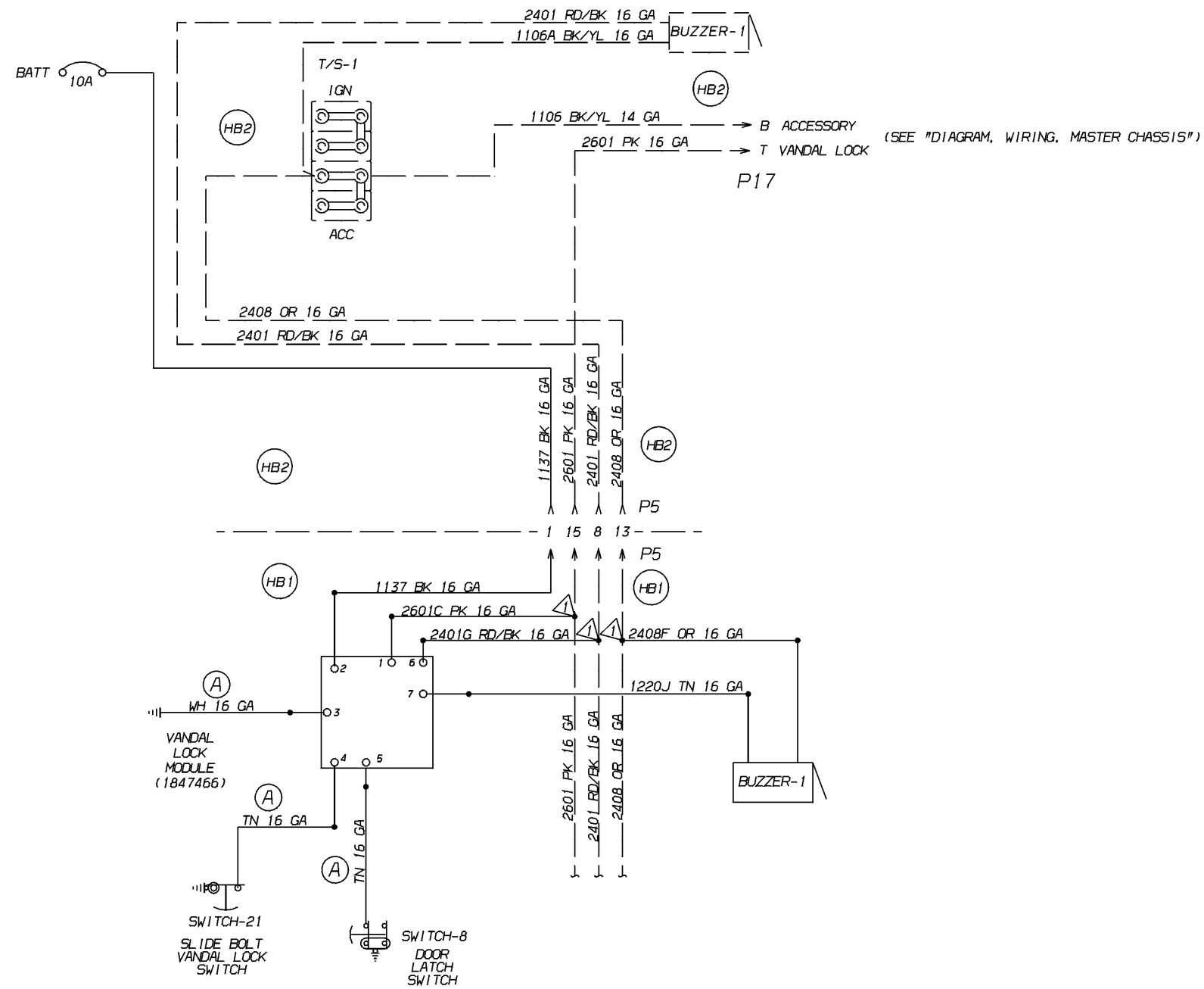
Vandal Lock for Left Side Emergency Door w/Sliding Bolt, Feature 0219-03 w/31201-05 0028528 A
