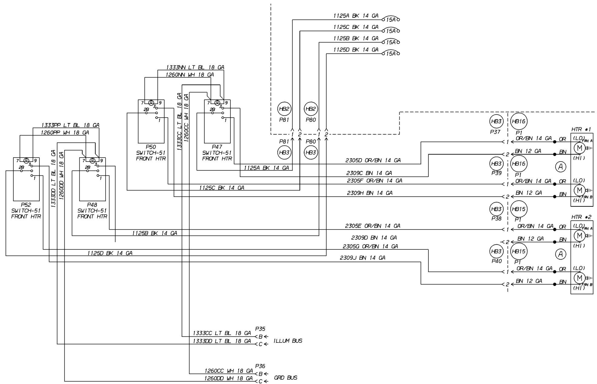
80,000 BTU Front LH Underseat Heaters, 0027189 A
