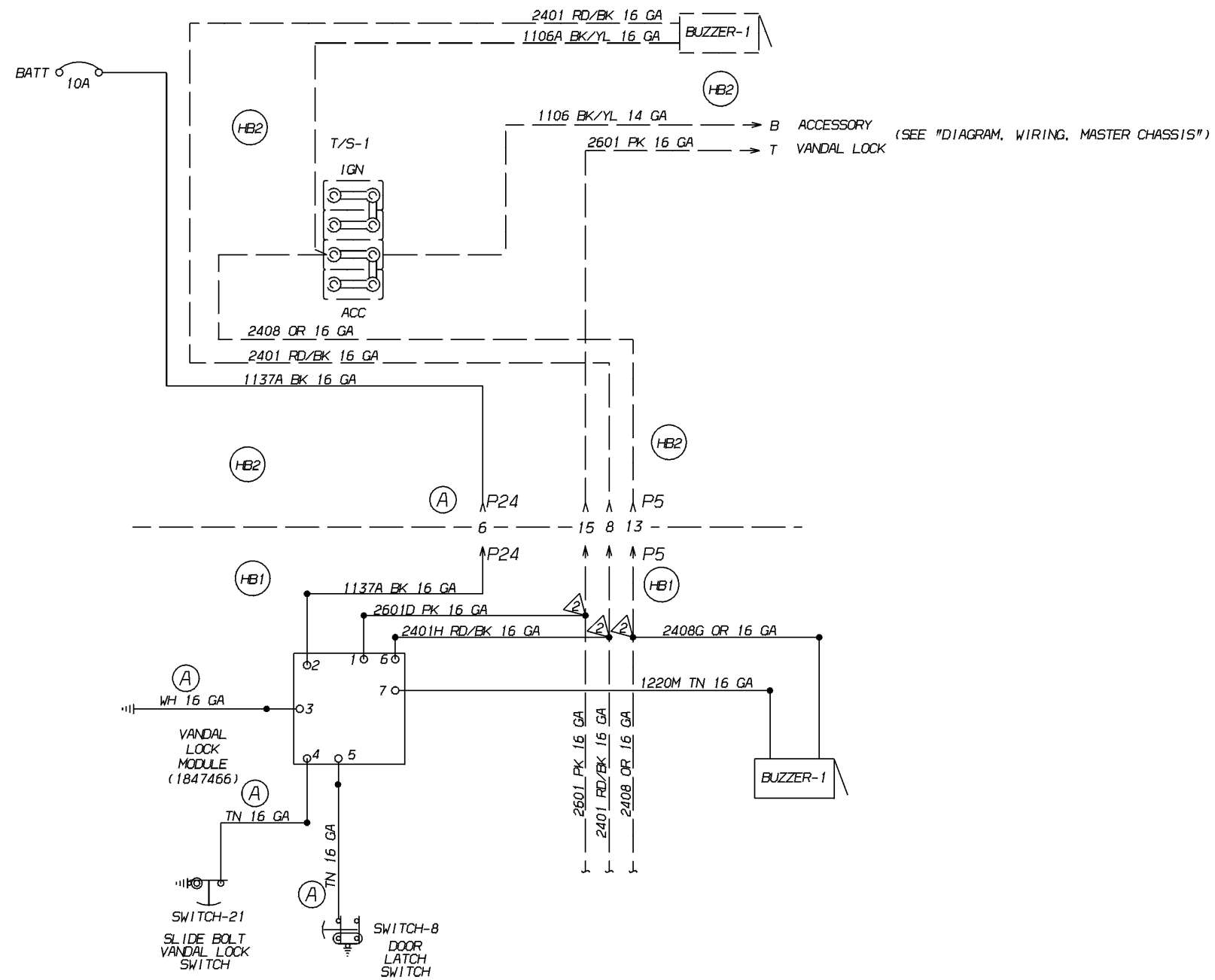
Vandal Lock for Right Side Emergency Door w/Sliding Bolt, Feature 0219-03 w/31201-06, 0028529 A
