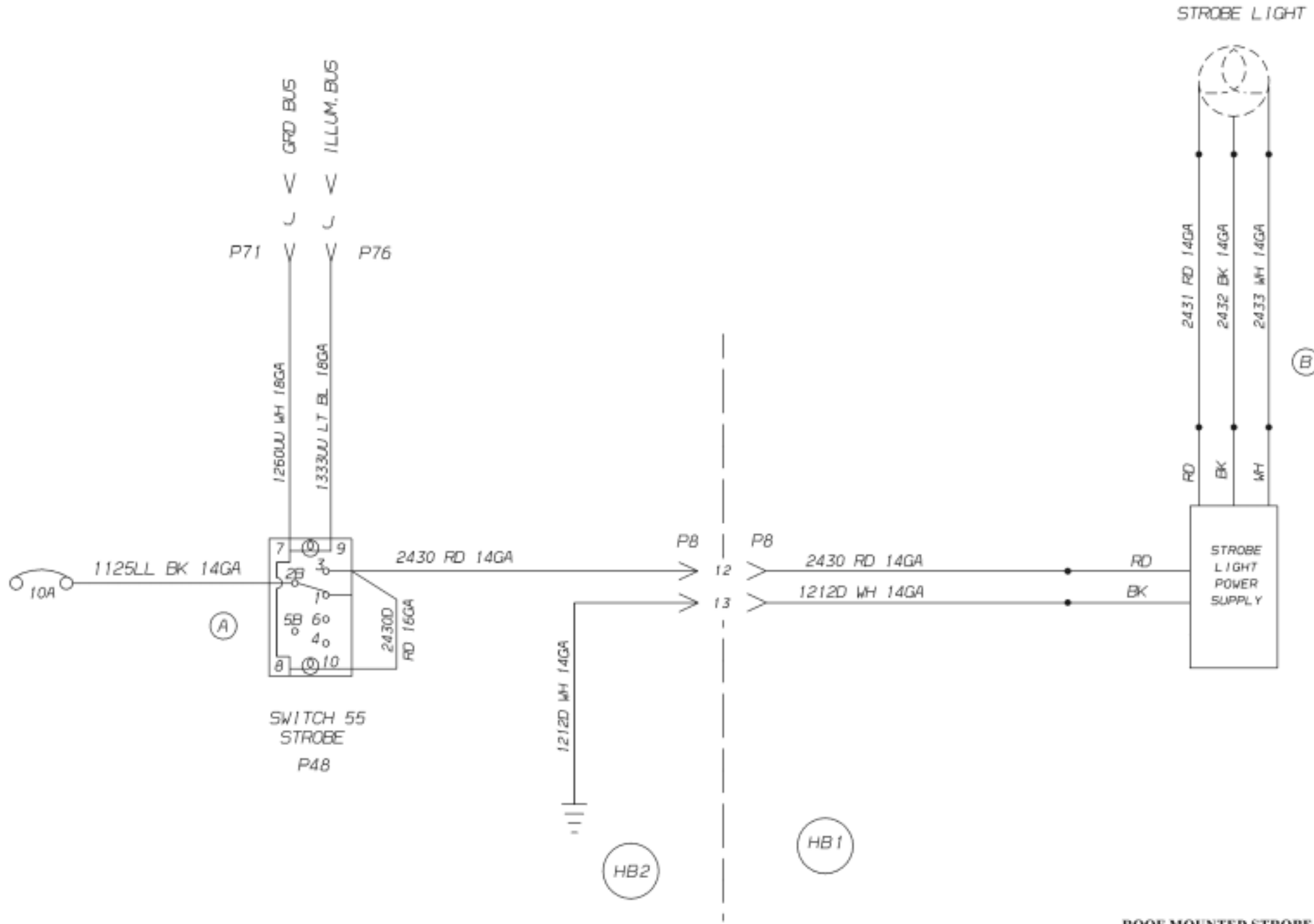
ROOF MOUNTED STROBE LIGHT 0028512 B
