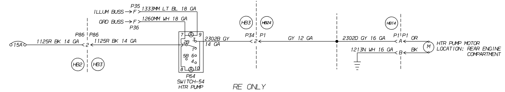
Heater Pump, Feature 30058-01, 02, 0027194
