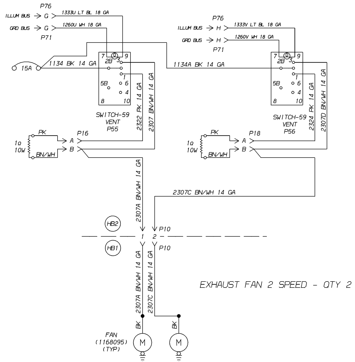
Exhaust Fan, 2 Speed, Feature 0551, 0027814
