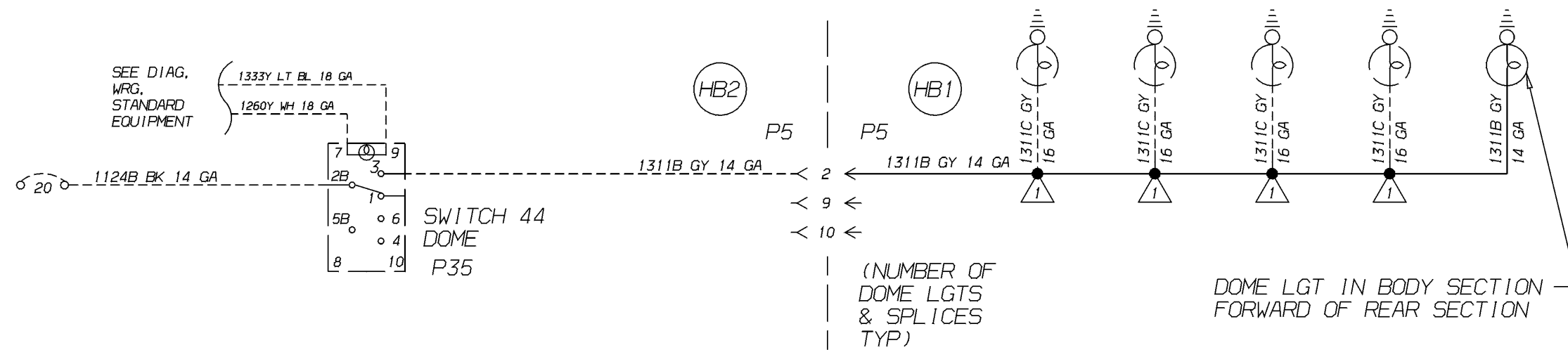
FEA 30158-04 WIRING, DOME, 1 ADDITIONAL, REAR, CENTERED
