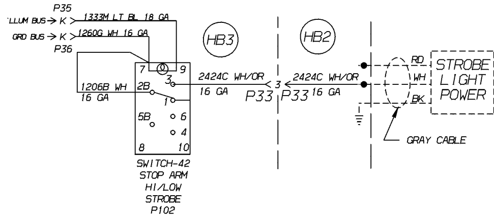
FEA 30297-03 STOP ARM, HI-LO, STROBE CNTL (WRG) W/30295-03 LOC, FRT W/30210-14 LOC, RH
