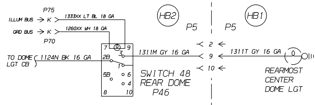
FEA 30157-01 WIRING, DOME, RR SW, 1 LGT
