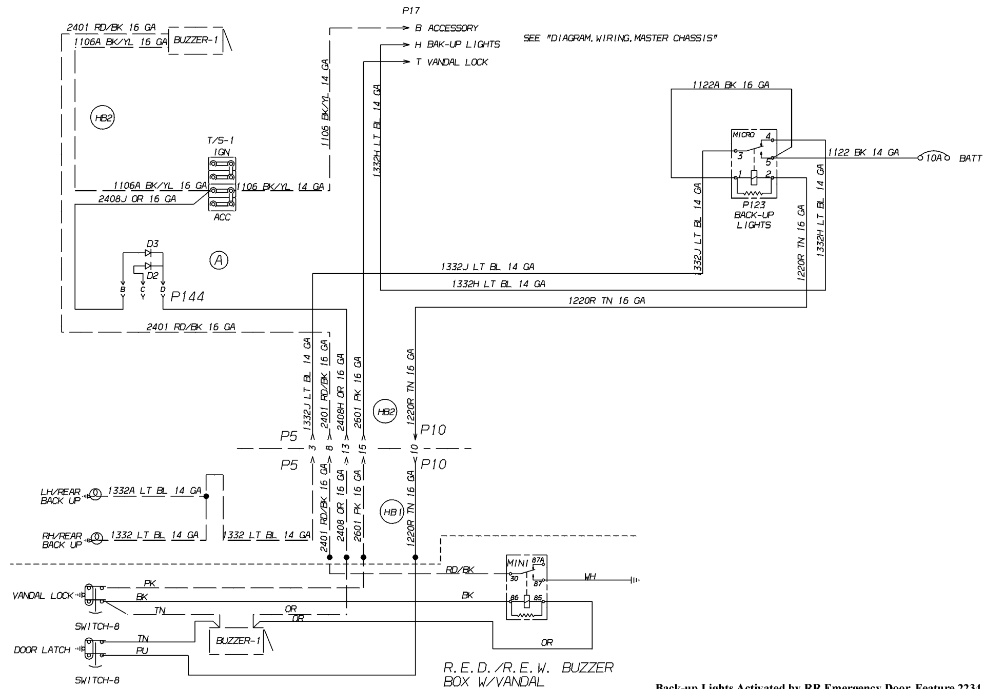
Back-up Lights Activated by RR Emergency Door, Feature 2234, w/0217, 0219 0028526 A
