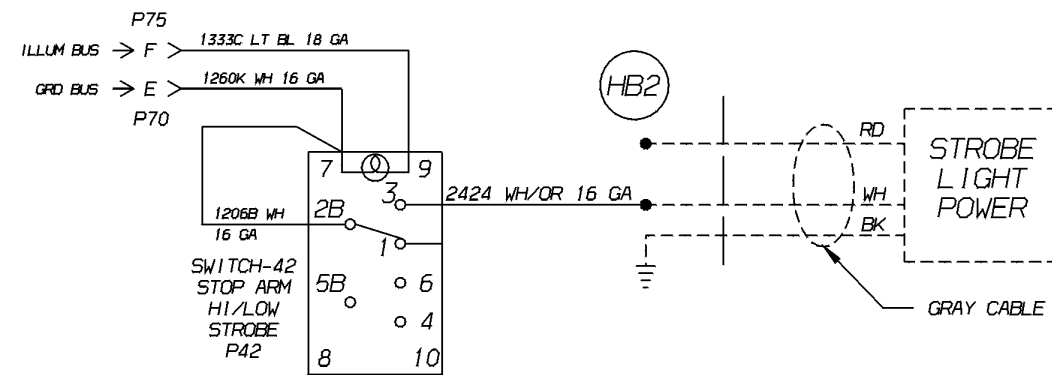
FEA 30297-03 STOP ARM, HI-LO, STROBE CNTL (WRG) W/30295-03 LOC, FRT W/30210-13 LOC, LH
