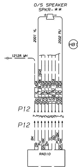
30269-07 WIRING & SPEAKER, O/SIDE, ROOF, LH, YELLOW 30269-08 WIRING & SPEAKER, O/SIDE, ROOF, LH, GRAY ** 30269-07 - SPKR-4 30269-08 - SPKR-3
