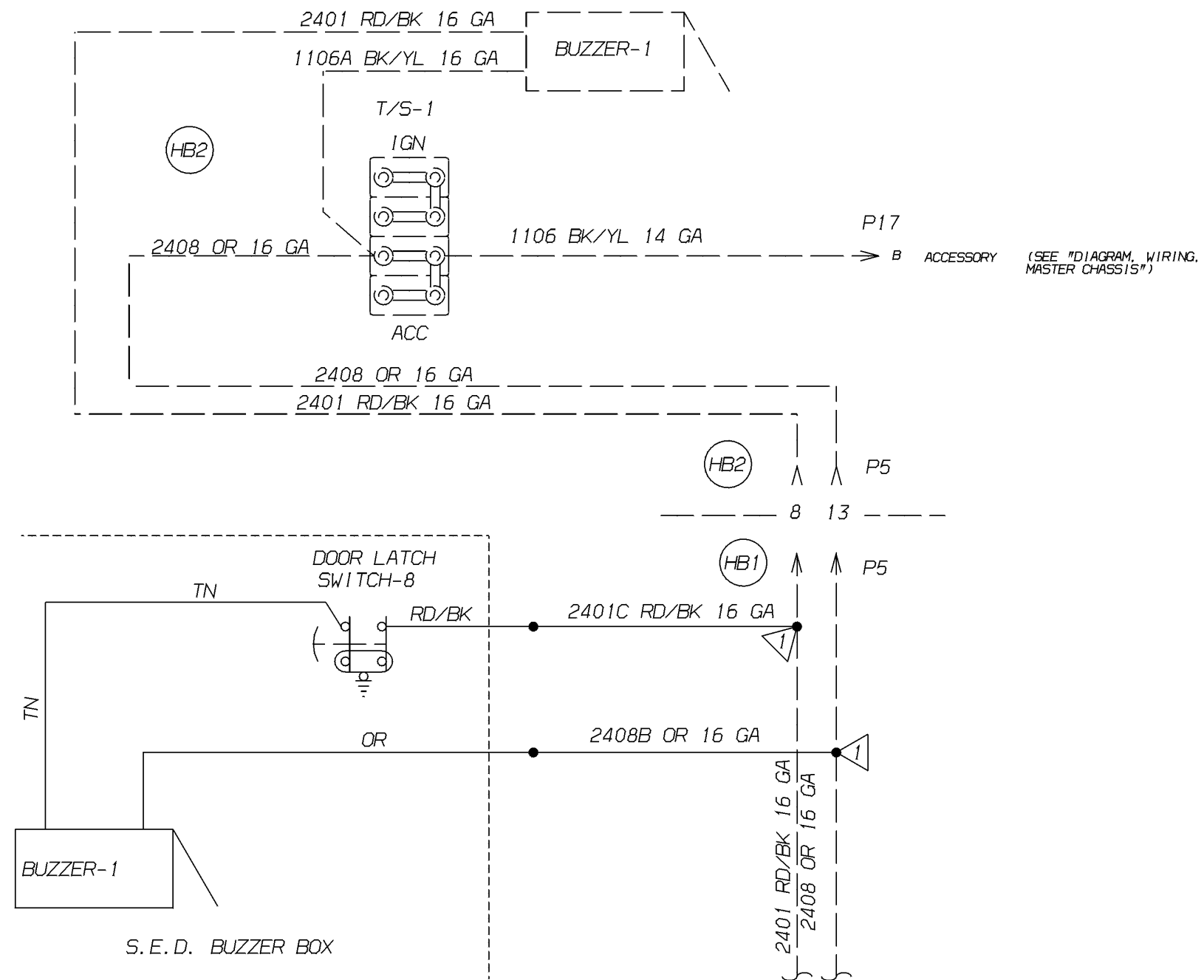
Left-Hand Side Emergency Door, Feature 31201-05, 0028524 A
