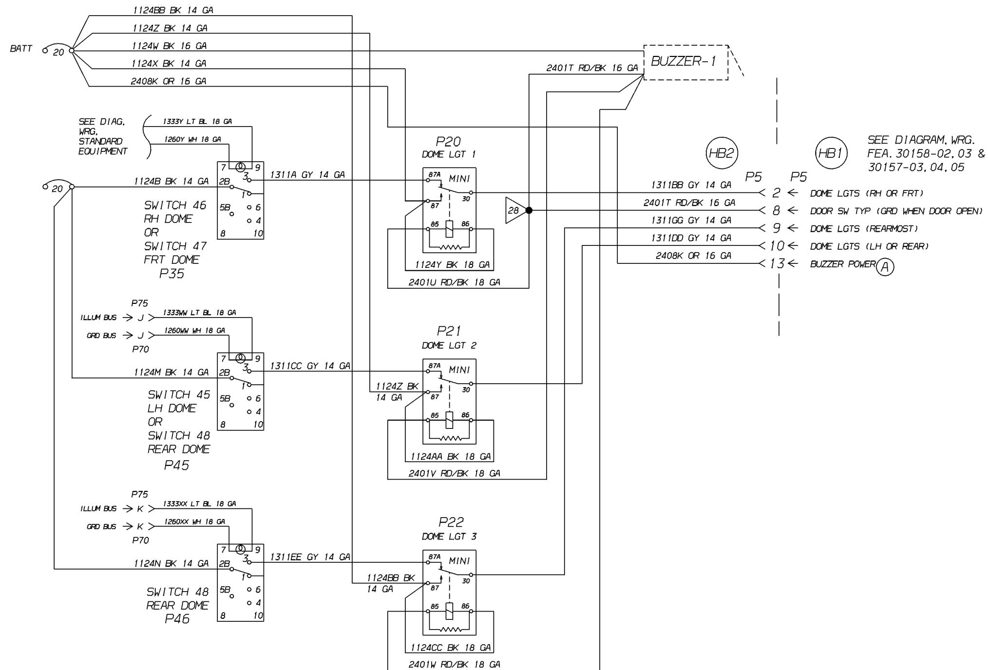
Dome Lights Activated by Emergency Exits, Feature 6689-03 w/30158, 30157, 0027785 A
