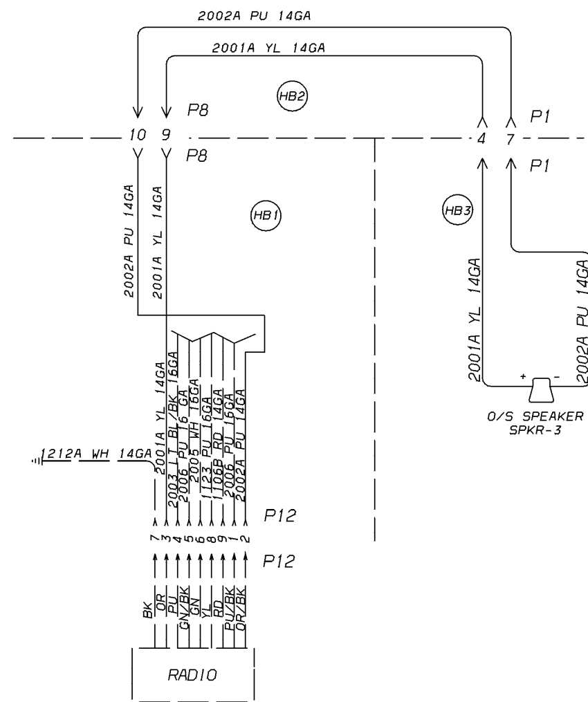
30269-10 WIRING & SPEAKER, O/SIDE, U/FLOOR, RH
