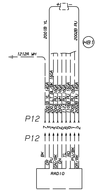
30269-09 WIRING, W/O SPEAKER, RH ROOF AREA (SPEAKER NOT INCLUDED)
