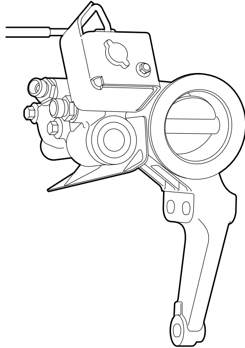
EGR valve with actuator
