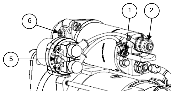
28MT or 29MT STARTER
