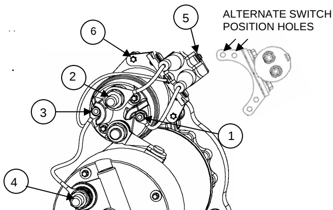
37MT, 41MT or 42MT STARTER
