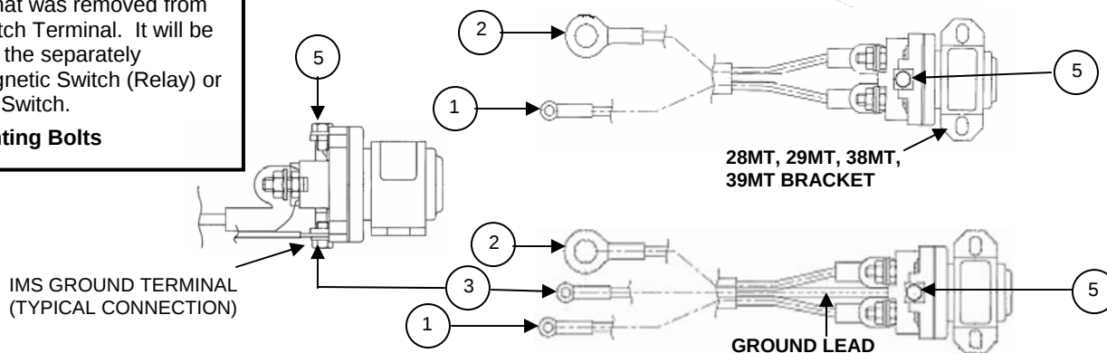
GROUND LEAD
