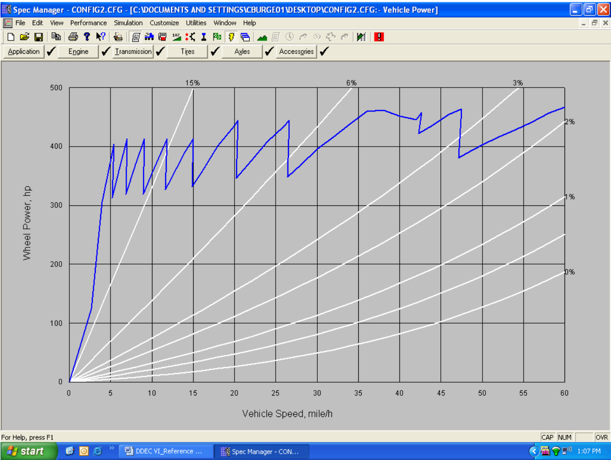
Vehicle Power Graph
