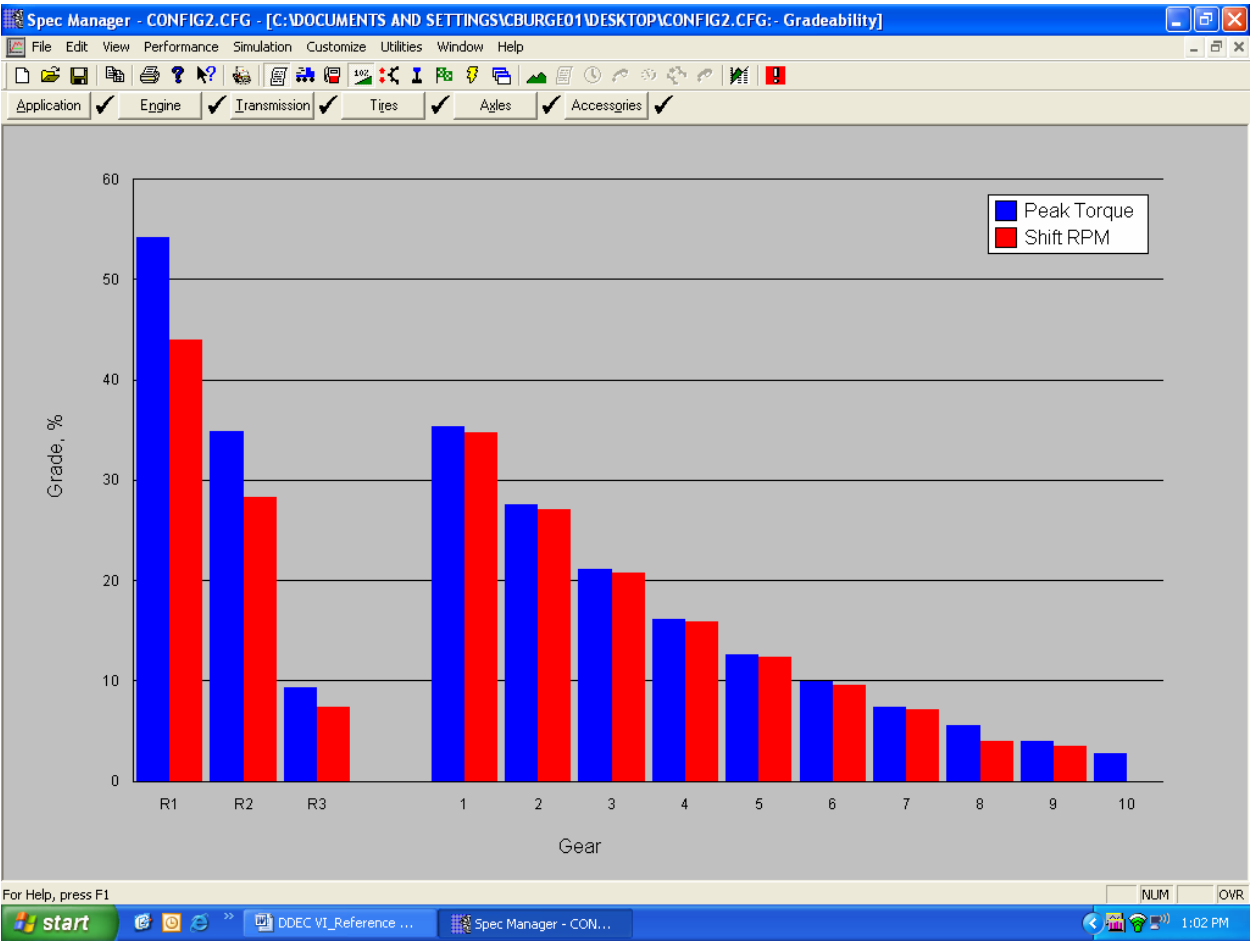
Gradeability Graph
