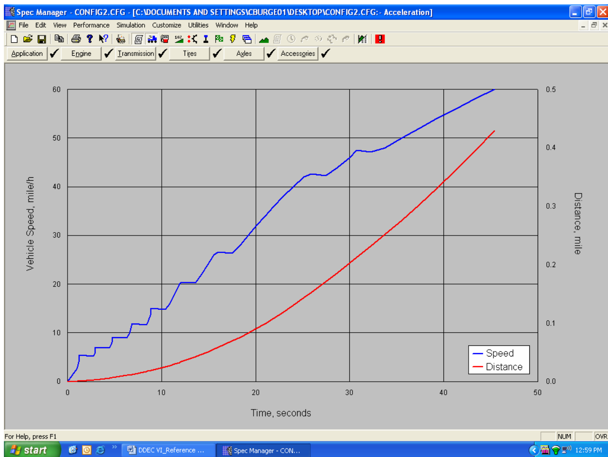
Acceleration Graph
