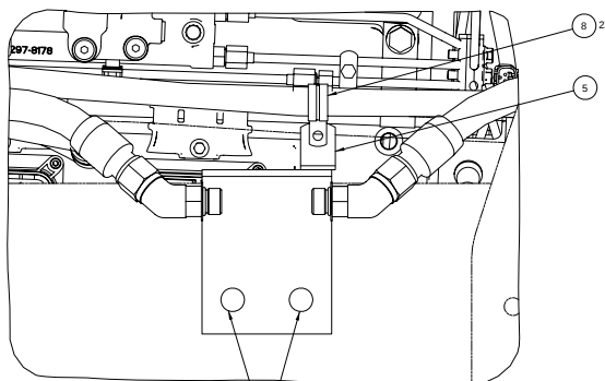
V95-1081-1: ROUTING WITHOUT FUEL COOLER
