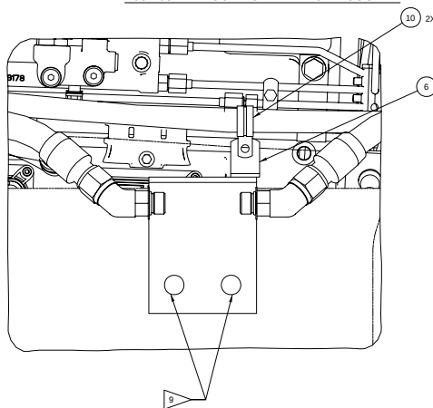
V95-1081-2: ROUTING WITH FUEL COOLER
