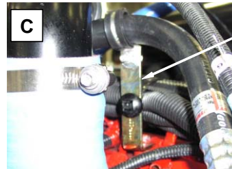
K028-867 STANDOFF USED TO SUPPORT A/C LINE AND ALTERNATOR HARNESS
