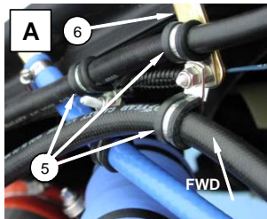
VIEW SHOWING STANDOFF ATTACHER TO COOLING MODULE
