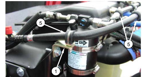
VIEW SHOWING RECEIVER DRYER DETAILS RECEIVER DRYER MOUNTED ON COOLING MODULE
