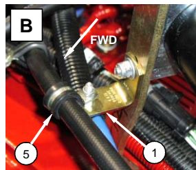
VIEW SHOWING STANDOFF ATTACHED TO UPPER RADIATOR PIPE SUPPORT
