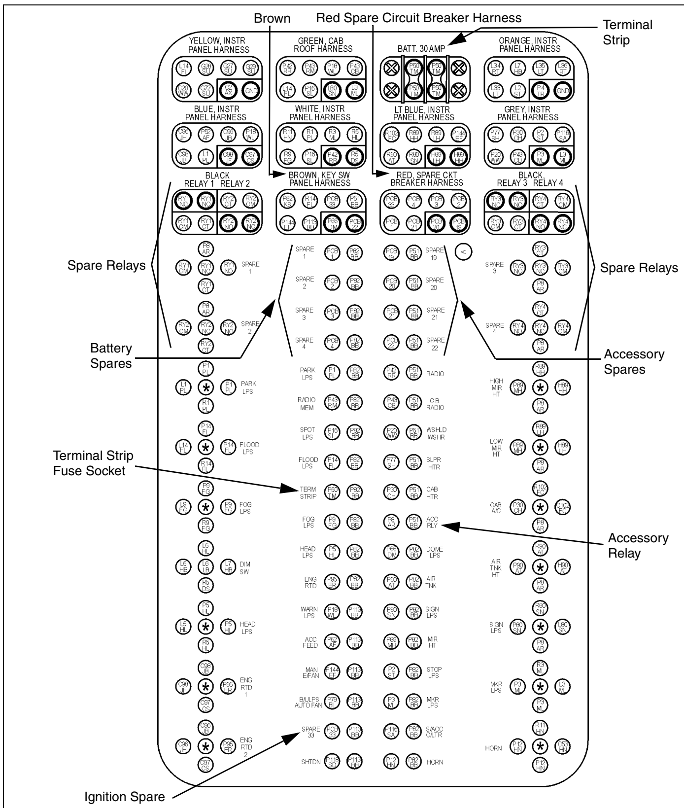
Figure 3 Power Distribution Box
