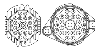
CIRCUIT POSITION CHART:
