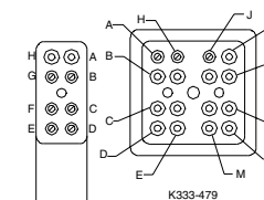
CIRCUIT POSITION CHART:
