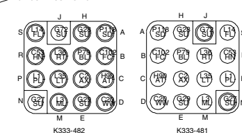
CIRCUIT POSITION CHART:
