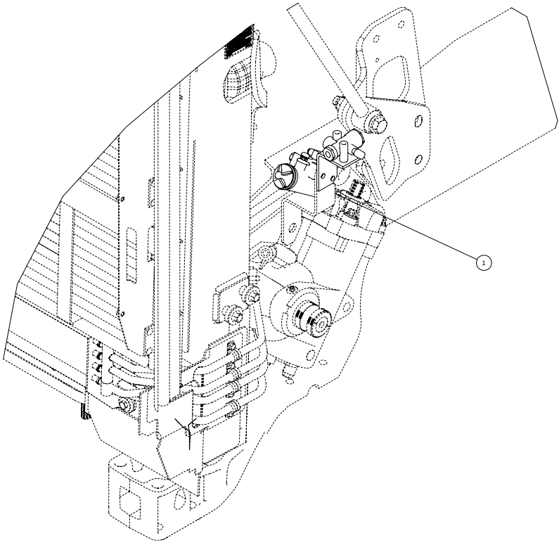
G97-1102-004 FOR USE WITH BENDIX CT596 T8W W/ BEHR MODULE (PARTS NOT ID'D ARE SAME AS G97-1102-002)
