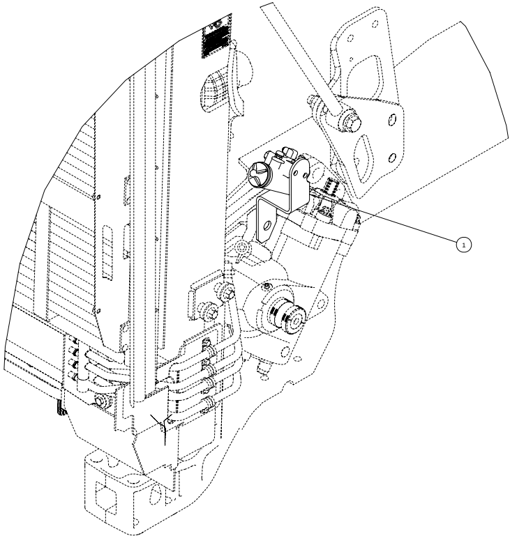
G97-1102-003 FOR USE WITH ALL AIR COMPRESSORS EXCEPT BENDIX CT596 T8W W/ BEHR MODULE (PARTS NOT ID'D ARE SAME AS G97-1102-001)
