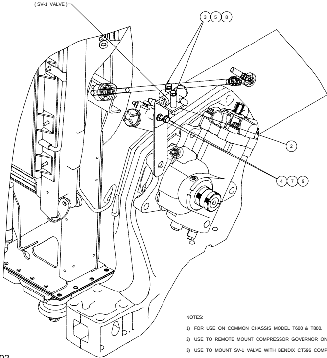
G97-1102-002 FOR USE WITH BENDIX CT596 NOT T8W W/ BEHR MODULE (PARTS NOT ID'D ARE SAME AS G97-1102-001)
