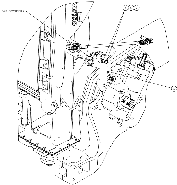
G97-1102-001 FOR USE WITH ALL AIR COMPRESSORS EXCEPT BENDIX CT596 NOT T8W W/ BEHR MODULE
