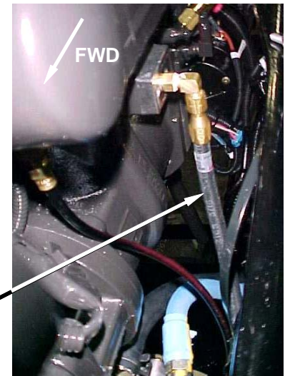
VIEW SHOWING HOSE AT COMPRESSOR
