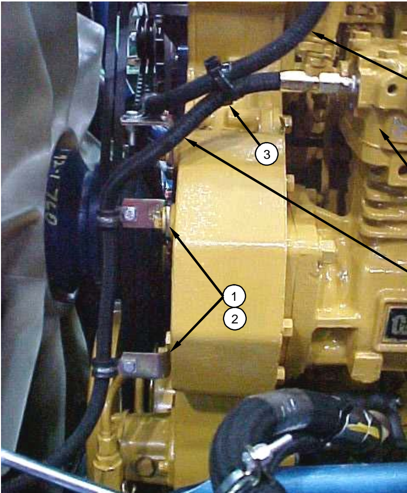
VIEW SHOWING L.H. SIDE OF ENGINE
