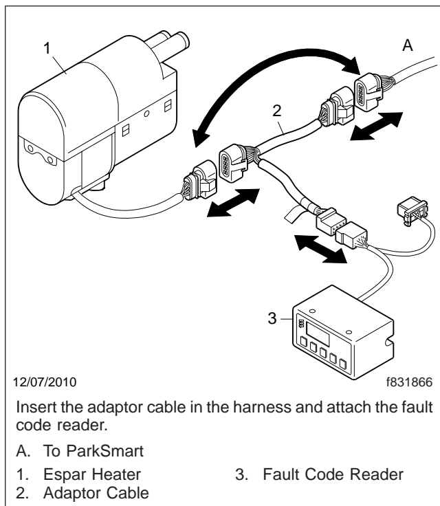
Fig. 4, Adaptor Cable and Fault Code Reader
