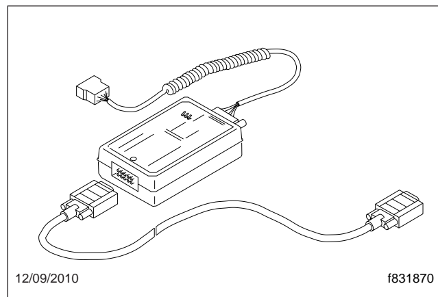
Fig. 5, EDiTH Diagnostic Tool
