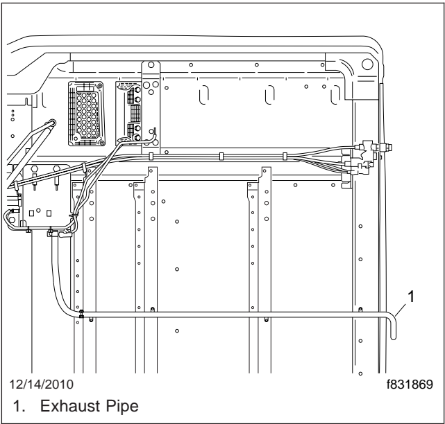
Fig. 7, Exhaust Pipe Installation
