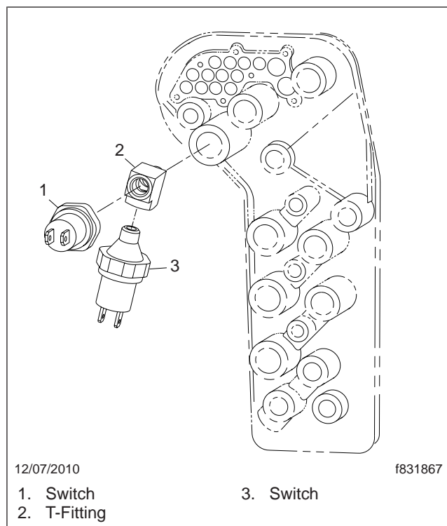
Fig. 9, Park Brake Pressure Switch Location (typical)
