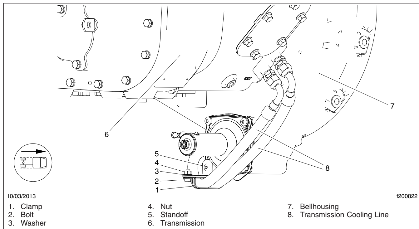
Fig. 8, Transmission Cooler Line and Bracket Installation
