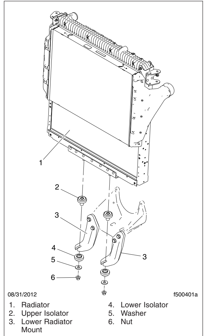
Fig. 15, Radiator Installation
