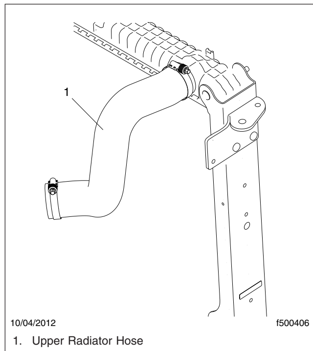
Fig. 17, Upper Radiator Hose Installation
