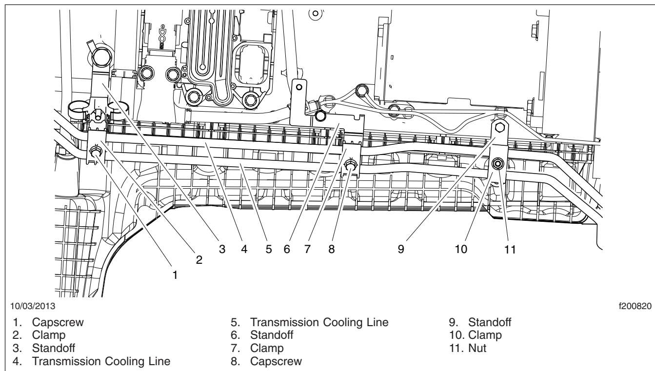
Fig. 7, Transmission Cooler Line Bracket Installation
