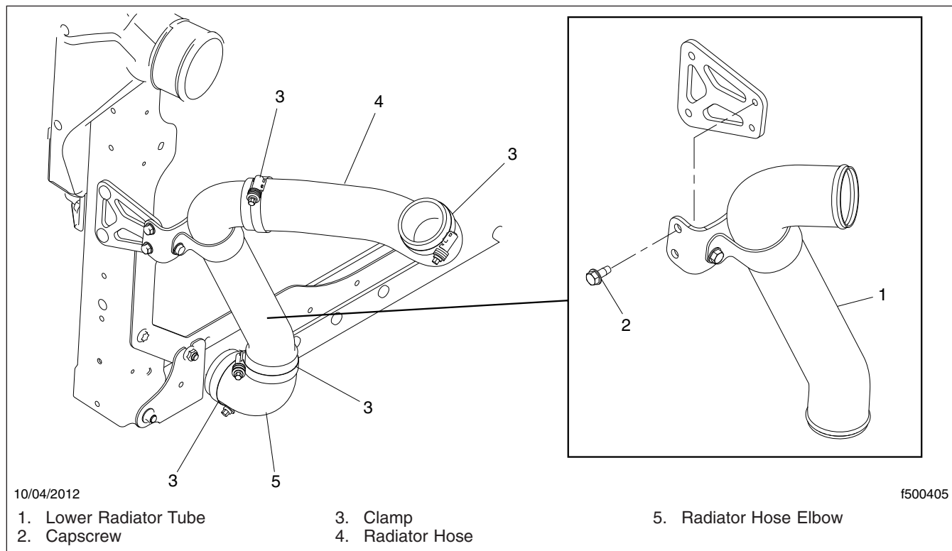
Fig. 18, Lower Radiator Hose Installation
