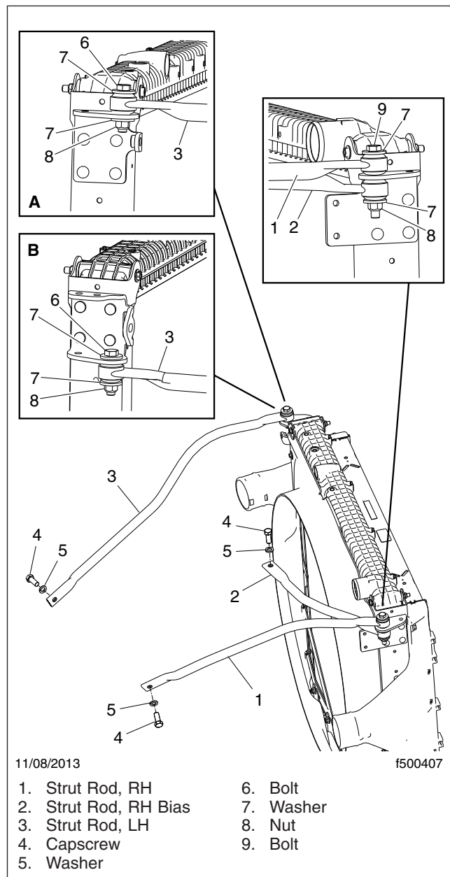
Fig. 16, Isolated Radiator Strut Rod Installation
