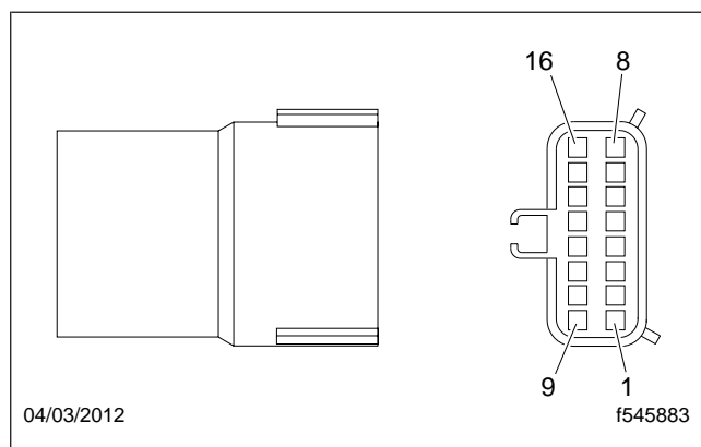
Fig. 1, Standard Transmission Interface Connector
