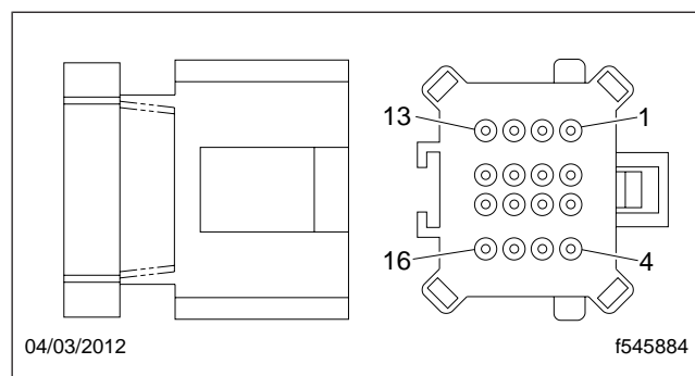
Fig. 2, Alternate Transmission Interface Connector
