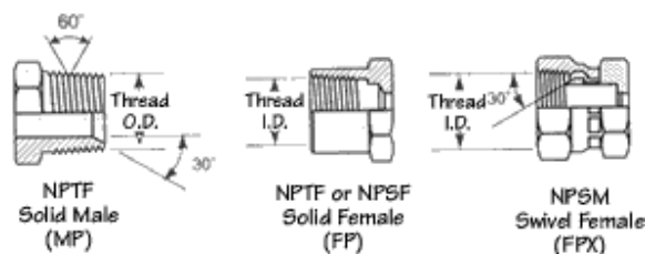
NPT Pipe Thread
