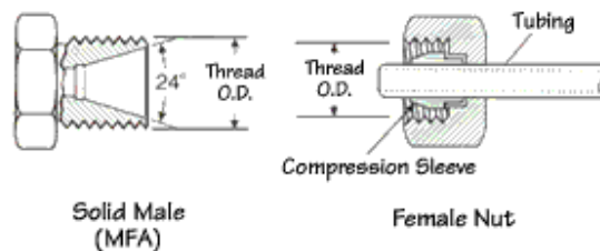
Flareless Tube
