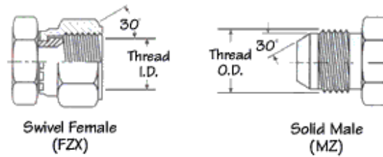
Parker Triple Thread Flare Fittings
