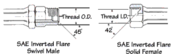
SAE Inverted Flare
