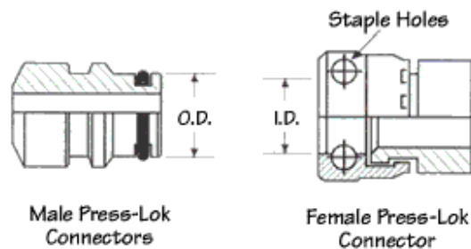
Press-Lok Connectors
