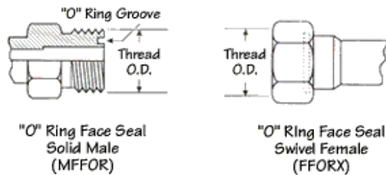
O-Ring Face Seal
