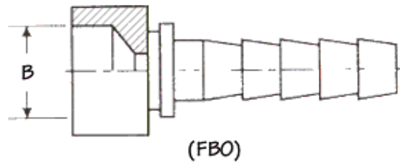
Braze-On Stems
