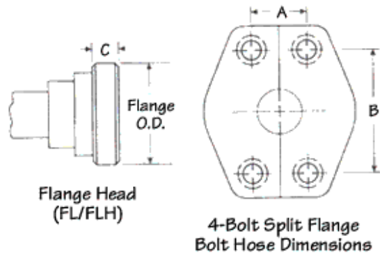
SAE Code 61 and Code 62
